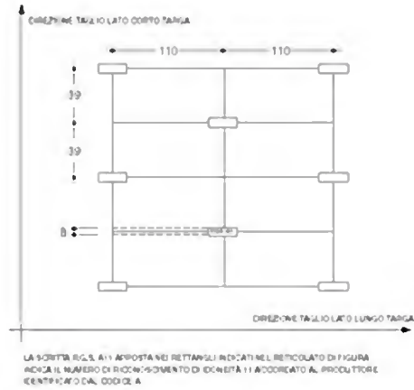
Figura III 6 Appendice IX Art. 260
