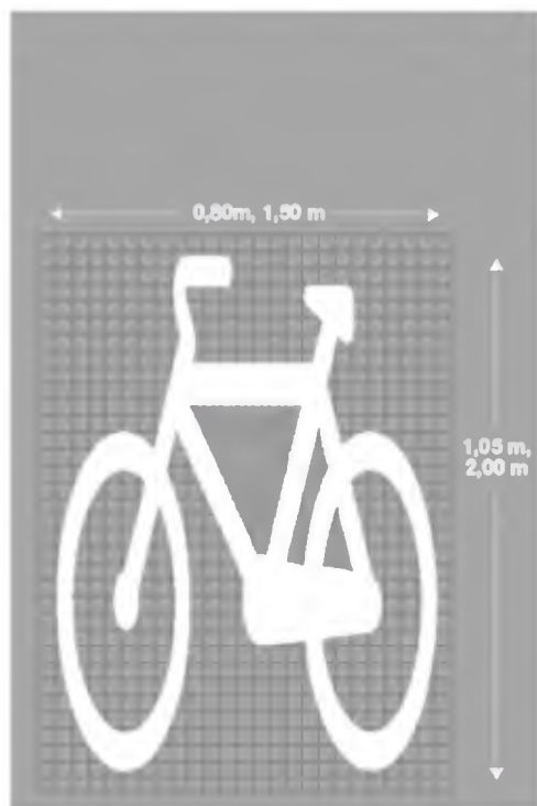
Figure II.443 Art. 148 - II.444 Art. 149
