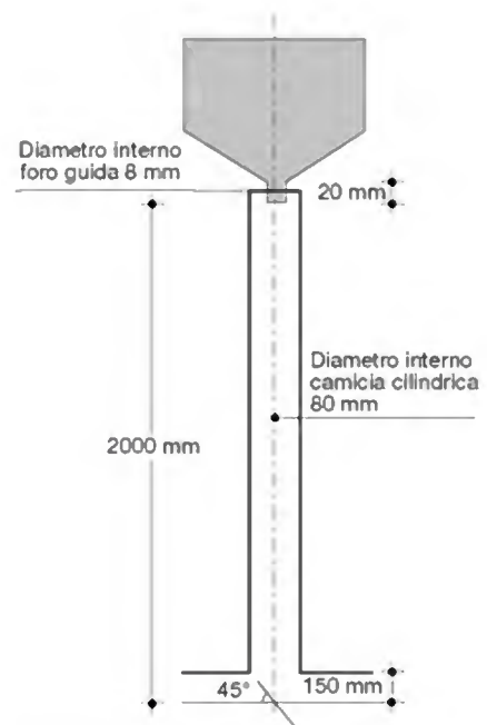
Figura III 8 Appendice IX Art. 260
